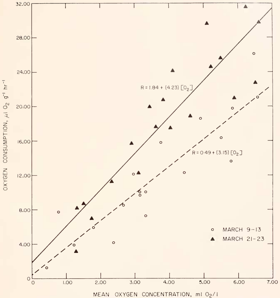
FIGURE 1. Oxygen consumption of Abarenicola pacifica as a function of oxygen concentration.
